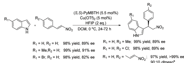
Scheme 42 Asymmetric Friedel–Crafts alkylation using a Cu-(S,S)-PyMBTH catalyst. a 10 mol% catalyst ( \text{Cu}(\text{OTf})_2 /(S,S)-PyMBTH = 1:1.1); double alkylation occurred.
