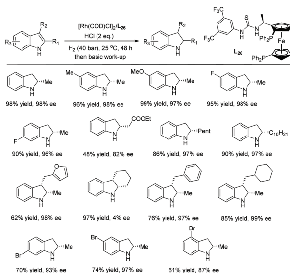
Scheme 52 EH of indoles using an \text{Rh}-\text{L}_{26} catalyst.
