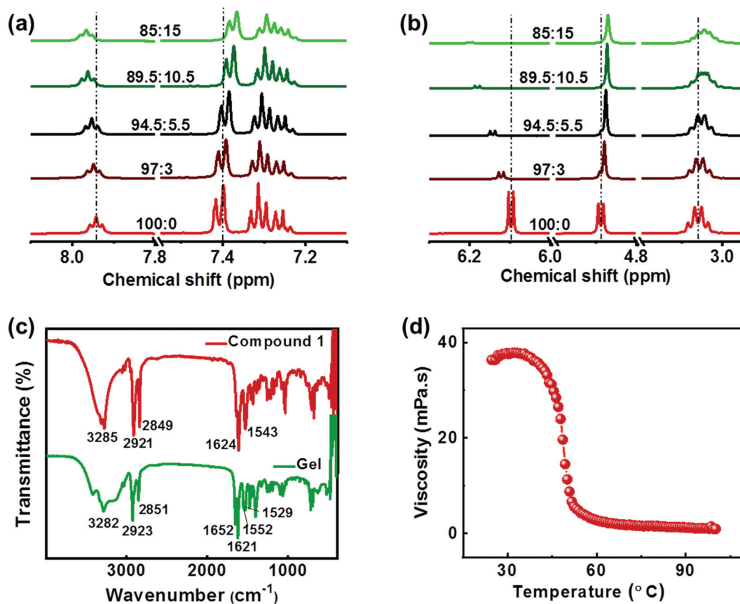
Fig. 3 (a and b) ^1\text{H} NMR spectral shifts observed upon stepwise addition of \text{D}_2\text{O} to \mathbf{1R} dissolved in \text{DMSO}-d_6 . The spectral shifts corresponding to (a) NH and aromatic protons, and (b) OH, chiral CH and aliphatic protons. (c) FT-IR spectra of crude (red trace) and the lyophilised gel (green trace) of \mathbf{1R} . (d) Temperature dependent viscosity changes of gel formed from \mathbf{1R} (4 wt%) in a binary solvent mixture of DMSO and water (4 : 1).
