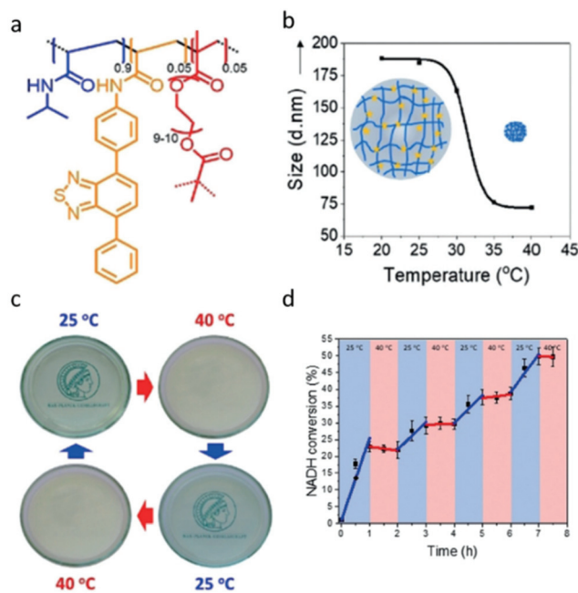
Fig. 4 (a) Photocatalytic temperature-responsive nanogels structure. (b) Temperature-dependent size of nanogels. (c) Reversible phase changes by changing temperature. (d) Temperature-dependent photocatalytic conversion of the enzyme cofactor NADH to NAD + . Reproduced from ref. 52 with permission from John Wiley and Sons, copyright 2019.
