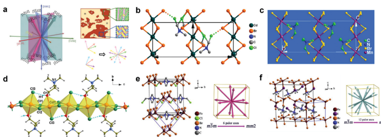
Fig. 5 Different structures of multi-axial ferroelectric halide perovskites. (a) Demonstration of twelve different polarization directions of the TMCM-MnCl 3 perovskite and the corresponding experimental evidence from PFM measurements. Reproduced with permission from ref. 48. Copyright 2017, American Association for the Advancement of Science. (b) Crystal structure of [(CH 3 ) 3 NCH 2 Cl]CdBr 3 in the ferroelectric phase. The dashed lines represent the Cl-Br interactions. Reproduced with permission from ref. 72. Copyright 2018, American Chemical Society. (c) Crystal structure of [(CH 3 ) 3 NCH 2 X]MnBr 3 in the ferroelectric phase. Reproduced with permission from ref. 73. Copyright 2017, American Chemical Society. (d) Crystal structure of [Me 3 NCH 2 CH 2 OH]CdCl 3 with the edge-sharing CdCl 5 O octahedra structure. The cations are coordinated alternatively above and below the perovskite framework. Reproduced with permission from ref. 74. Copyright 2020, American Chemical Society. (e) Crystal structure of (TMCM)FeBr 4 and the corresponding six equivalent polarization directions. (f) Crystal structure of (TMIM)FeBr 4 and the corresponding twelve equivalent polarization directions. Reproduced with permission from ref. 75. Copyright 2020, Elsevier.
