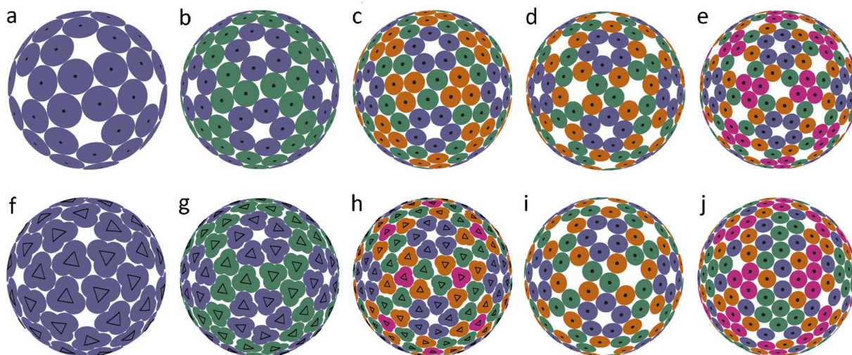
Fig. 2 Dense packings of disks and model trimers. The equilibrium spherical structures obtained by minimizing the interaction energy of point particles (represented by small black circles), which interact with each other with the l^{-200} pair potential. (a–e) Icosahedral packings of disks. Different colors denote different 60-fold orbits of the symmetry group I . (f–h) Icosahedral packings of particles rigidly bound into symmetrical trimers. Ratios r/R for these cases are: 0.12, 0.08, and 0.004, while the packings consist of 60, 120 and 180 trimers, respectively. (i and j) Packings arising from (d and e) when the requirement of icosahedral symmetry is removed.
