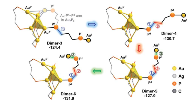
Scheme 2 Illustrative diagram for the structural tautomerization of the transformation of Dimer-3 to Dimer-6 (the relative energies are given in kcal mol -1 ). The alloy block away from Au 5 was omitted for clarity reasons.
