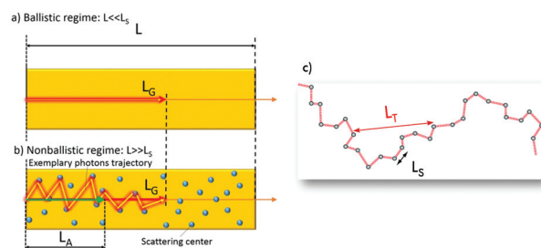
Fig. 3 Schematic of (a) ballistic and (b) non-ballistic regime ( L is the size of the random medium (for example its length in 1D), L_G and L_A are the gain and amplification lengths respectively). (c) Representation of length scales ( L_T and L_S are transport and scattering mean free paths respectively). ((a) and (b) is reproduced from ref. 31, with permission from [John Wiley and Sons]).
