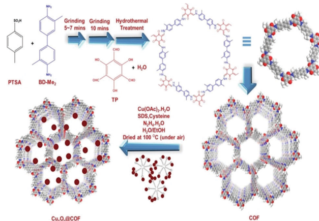
Scheme 10 A schematic diagram of the synthesis of \text{Cu}_x\text{O}_y@COF . Reproduced with permission from ref. 26; copyright: 2019, Journal of CO 2 Utilization.
