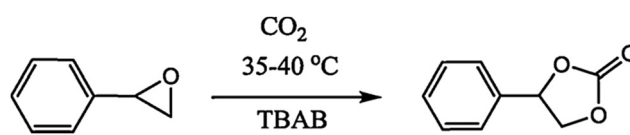
Scheme 11 The cycloaddition of CO 2 with styrene oxide using \text{Cu}_x\text{O}_y@COF . Reproduced with permission from ref. 26; copyright: 2019, Journal of CO 2 Utilization.
