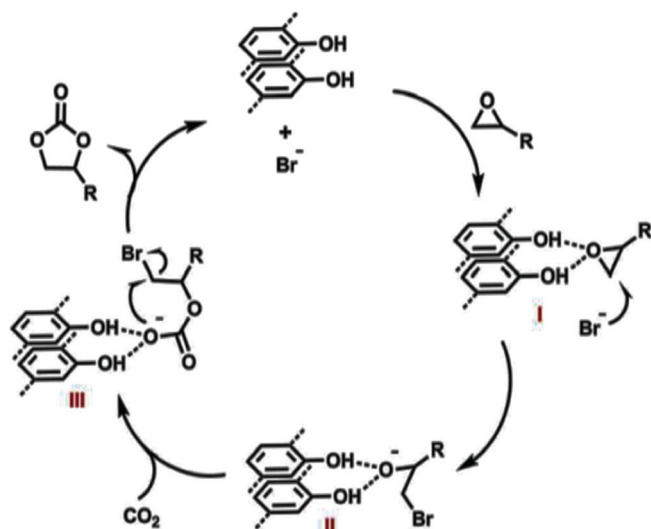
Scheme 9 A self-explanatory mechanistic path supporting the cycloaddition of CO 2 using COF-JLU7 and TBAB. Reproduced with permission from ref. 25; copyright: 2018, Journal of Materials Chemistry A.
