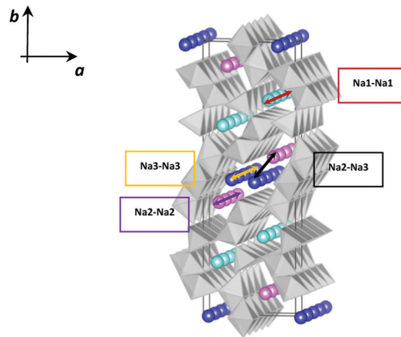
Fig. 2 Schematic representation of four possible \text{Na}^+ ion diffusion paths in \text{Na}_{0.44}\text{MnO}_2 ; Na1 cyan, Na2 pink, and Na3 blue.
