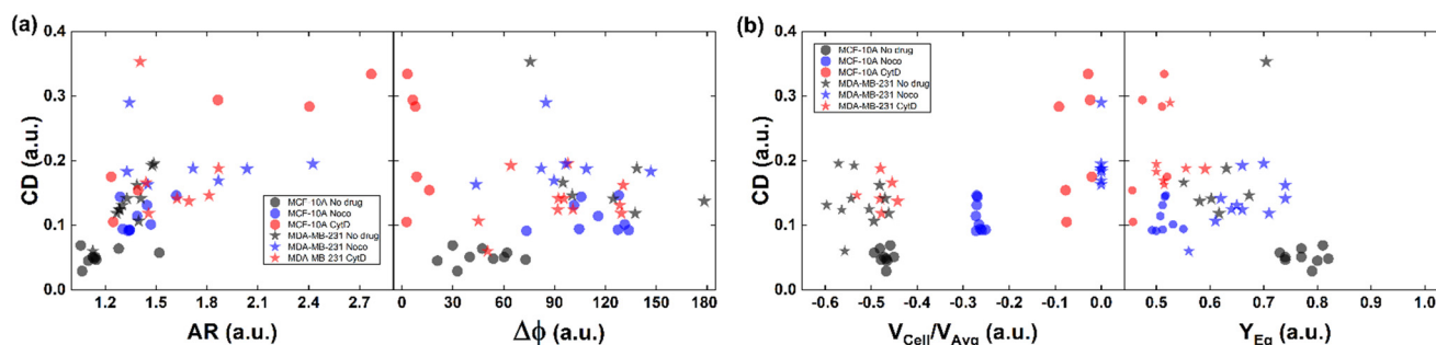
Fig. 4 CD variation with respect to AR, \Delta\phi , V_{Cell}/V_{Avg} , and Y_{Eq} for MCF-10A and MDA-MB-231 under no drug and treated conditions for each analysed cell. (a) CD variation with respect to AR and \Delta\phi is plotted for each cell. Increasing CD and AR are present for the treated cells. MCF-10A deforms more at CytD expressing lower values of \Delta\phi ( \leq 50^\circ ) related to a high CD range of (0.15–0.35) while MDA-MB-231 still shows 50^\circ \leq \Delta\phi \leq 180^\circ after CytD treatment, in the same range of no drug. MCF-10A deforms less at Noco expressing slightly equal values of \Delta\phi , AR and CD typical of a T motion. (b) CD variation with respect to V_{Cell}/V_{Avg} and Y_{Eq} is shown for each cell. It is verified that an increase of the CD values corresponds to a decrease of the V_{Cell}/V_{Avg} since cells tend to move at the same velocity of the fluid, without lagging it anymore. According to the V_{Cell}/V_{Avg} changes, the Y_{Eq} values decrease as cells move faster towards the centre line ( Y_{Eq} \sim 0.5 ) as the CD increases. The total number of analysed cells N_{Tot} = 49 . The Kruskal–Wallis test performed on the experimental data is reported in Table S4.†
