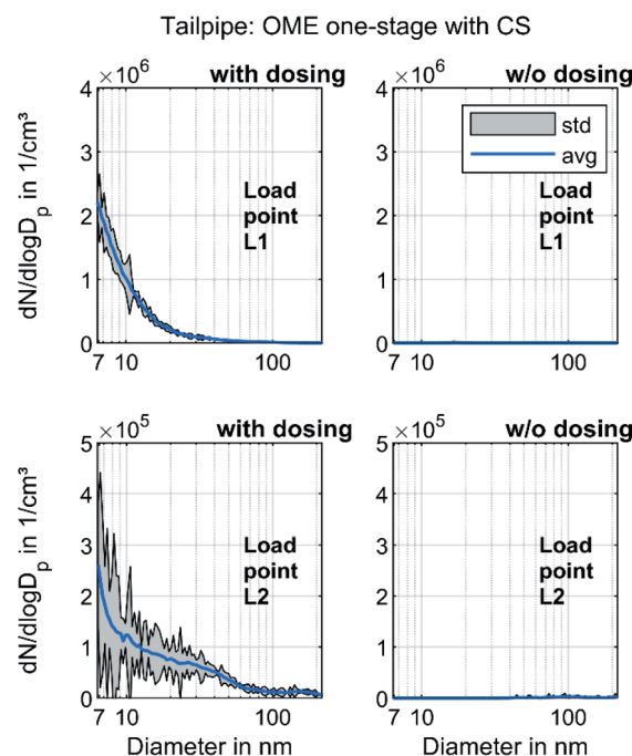
Fig. 7 Particle size distribution of OME tailpipe exhaust with and without urea dosing and one-stage dilution with volatile particle remover: filtered average (arithmetical mean) of three recordings and indication of the standard deviation.
