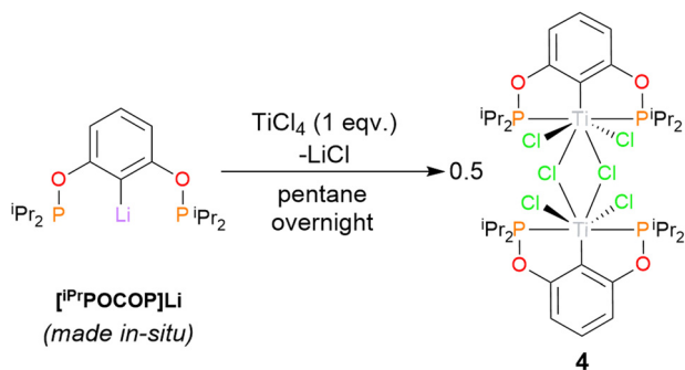
Scheme 5 Synthesis of 4 .
