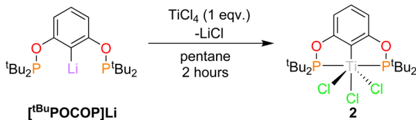
Scheme 3 Synthesis of 2 .
