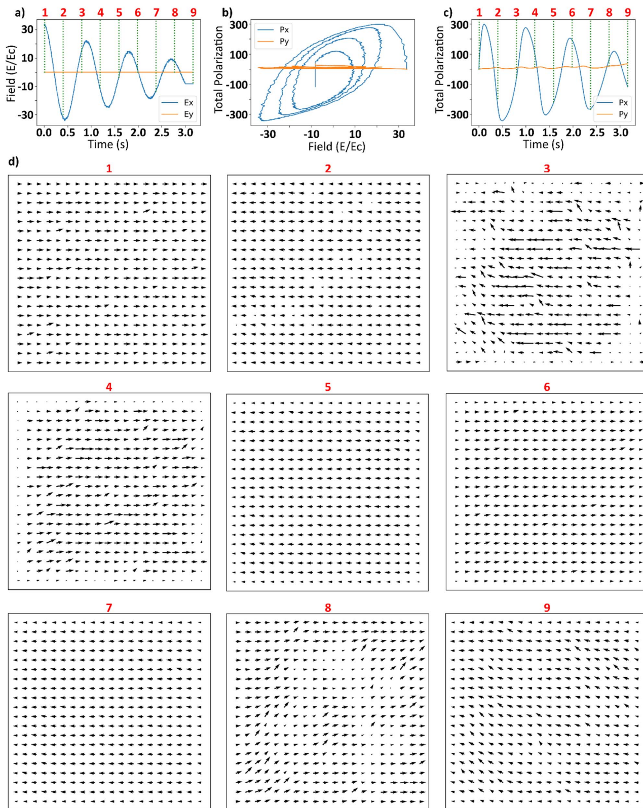
Fig. 5 (a) Applied external electric field as a proportion of coercive field of the system as a function of time. (b) Resulting polarization in x -direction and y -direction as a function of applied electric field in x -direction. (c) Resulting polarizations in x and y directions as a function of time. (d) The snapshots of polarization vectors at each lattice sites at uniform time intervals. Vertical green lines in (a) and (c) represent the time at which polarization maps in (d) are plotted.
