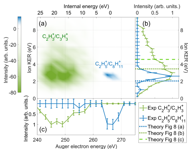
Fig. 9 The difference in energy-resolved AEPIICO data for the C_2H_3^+/C_3H_3^+ (green) and the C_2H_5^+/C_8H_{11}^+ (blue) ion pairs. (a) 2D map showing the energy correlation of the Auger electron energy with the total ion kinetic energy released (KER) for the selected ion pairs. The intensities of the C_2H_3^+/C_3H_3^+ events is set to be negative and the C_2H_5^+/C_8H_{11}^+ events is set to be positive for better contrast in the map. (b) The projection of (a) showing the experimental total ion KER of the C_2H_3^+/C_3H_3^+ (green) and the C_2H_5^+/C_8H_{11}^+ (blue) ion pairs. The theoretical ion KER values obtained from PES (Fig. 8) are shown as vertical dashed lines. (c) The projection of (a) showing the experimental Auger electron energy for the C_2H_3^+/C_3H_3^+ (green) and the C_2H_5^+/C_8H_{11}^+ (blue) ion pairs.
