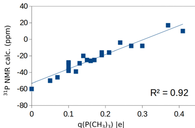
Fig. 4 Plot of computed ^{31}\text{P} chemical shift versus the Bader charge on \text{P}(\text{CH}_3)_3 adsorbed on various \text{M}^{4+} sites of \alpha\text{-TiO}_2 , \text{r-TiO}_2 , \text{ZrO}_2 , \text{SnO}_2 , and \text{CeO}_2 . We also include in the plot the free \text{P}(\text{CH}_3)_3 molecule, with chemical shift -60 ppm and q(\text{P}(\text{CH}_3)_3) = 0 .
