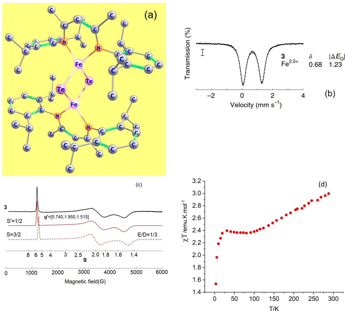
Fig. 2 Experimental X-ray structure of the mixed valence complex \text{Fe}^{2.5+}_{-\mu_2}\text{Te}_2\text{-Fe}^{2.5+} (a); its T = 80 K Mössbauer spectrum in zero magnetic field (b); continuous-wave X-band EPR spectrum (9.63 GHz) of a frozen solution at 3.6–8 K, collected under non-saturating microwave power conditions (black line) and simulations (red lines): pseudo-spin S' = 1/2 , g' = [5.740, 1.950, 1.515] (solid red line) and a S = 3/2 , spin-Hamiltonian, |D| \gg h\nu , |E/D| = 1/3 (assuming g = g_e = 2.0023 ) and a value of D < 15 \text{cm}^{-1} , estimated from the temperature dependence of the Lorentzian linewidth (c), variable-temperature SQUID magnetic susceptibility of a solid sample (d); data have been reproduced in a modified form from J. T. Henthorn, G. E. Cutsail III, T. Weyhermüller and S. DeBeer, "Stabilization of intermediate spin-states in mixed-valence diiron dichalcogenide complexes", Nat. Chem. , https://doi.org/10.1038/s41557-021-00853-5 .
