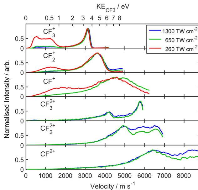
Fig. 6 P(v) distributions for the CF_n^{p+} ( n = 1-3, p = 1, 2 ) fragments derived from analysis of images obtained from SFI of CF_3I with \lambda = 805 nm photons at l = 1300, 650 and 260 TW\ cm^{-2} with, in each case, the strongest feature normalised to unit intensity. The corresponding KE_{CF_3} scale is shown on the top x-axis.
