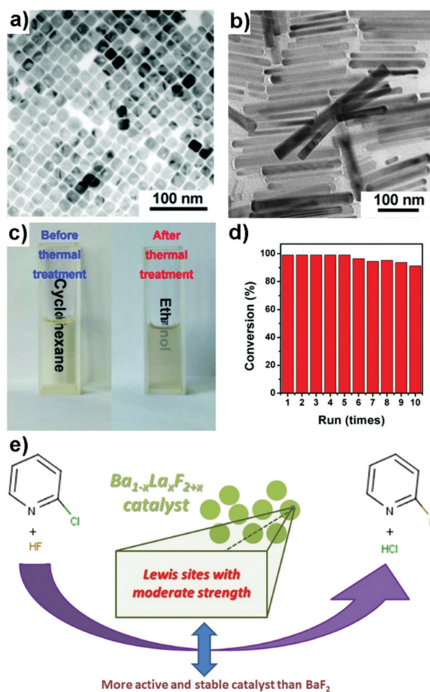
Fig. 6 TEM images of (a) \text{NaScF}_4 and (b) \text{KSc}_2\text{F}_7 nanocrystals. (c) Photograph of \text{NaScF}_4 nanocrystal solutions before and after thermal treatment at 500^\circ\text{C} under \text{Ar}/\text{H}_2 . (d) Reusability test of \text{NaScF}_4 nanocrystals for 10 cycles in the cyanosilylation reaction. 96 Reprinted with permission from ref. 96. Copyright 2017, Royal Society of Chemistry. (e) A scheme for the gas phase fluorination of 2-chloropyridine by HF using \text{Ba}_{1-x}\text{La}_x\text{F}_{2+x} . 97 Reprinted with permission from ref. 97. Copyright 2017, Elsevier.
