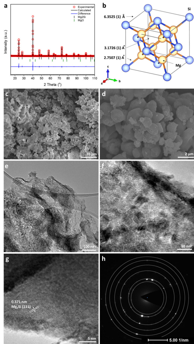
Fig. 1 Results from PXRD and electron microscopy for the MIMP-synthesised \text{Mg}_2\text{Si} powders, showing (a and b) profile plot of the Rietveld refinement against PXD data and the corresponding crystal structure; (c and d) SEM images, (e–g) TEM images, and (h) SAED pattern taken from the area shown by the image in (g).
