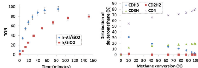
Fig. 4 Monitoring catalytic H/D exchange of methane. Left: Turnover number as a function of reaction time for catalysts Ir-Al/SiO 2 and Ir/SiO 2 at 250 ^{\circ} C and 0.67 mol% Ir surface sites. Right: Distribution of deuteromethanes as a function of CH 4 conversion for Ir-Al/SiO 2 .
