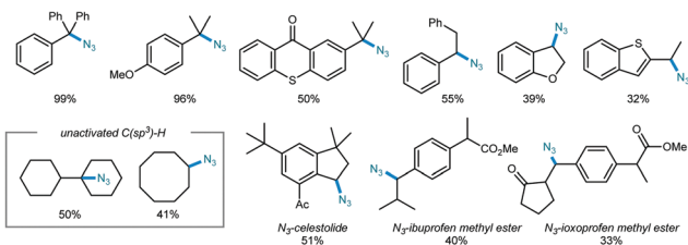
Scheme 22 Manganese catalyzed oxidative azidation of C(sp 3 )-H bonds via electrophotocatalysis.
