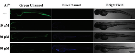
Fig. 5 Confocal fluorescence imaging of exogenous \text{Al}^{3+} in zebrafish. Top row: zebrafish were incubated with the probe BTM (5 \mu\text{M} ) for 60 min. Others: zebrafish were preincubated with 10, 20 and 50 \mu\text{M} \text{Al}^{3+} for 60 min and then incubated with the probe BTM (5 \mu\text{M} ) for 60 min, respectively. ( \lambda_{\text{ex}} = 405 \text{ nm} , \lambda_{\text{em}} = 440\text{--}500 \text{ nm} for the blue channel; \lambda_{\text{ex}} = 488 \text{ nm} , \lambda_{\text{em}} = 510\text{--}550 \text{ nm} for the green channel). Scale bar: 0.5 mm.
