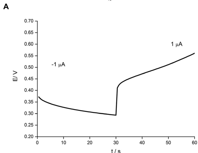
Fig. 3 (A) Nyquist plot and (B) chonopotentiometric cathodic/anodic curve ( \pm 1 \mu\text{A} ) for potassium-selective ISEs.
