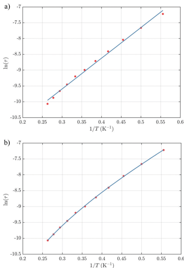
Fig. 6 Relaxation time of the magnetization \ln(\tau) vs. T^{-1} plot for 3 . (a) Arrhenius fitting with \ln(\tau) = \ln(\tau_0) + U_{\text{eff}}/T gives an effective blocking barrier of U_{\text{eff}} \approx 9.72 K and \tau_0 \approx 3.69 \times 10^{-6} s if only the Orbach process is used. (b) Arrhenius fitting \ln(\tau) = -\ln(\tau_0)^{-1} \exp(-U_{\text{eff}}/T) + CT^n gives an effective blocking barrier of U_{\text{eff}} \approx 8.39 K, \tau_0 \approx 1.45 \times 10^{-5} s, n = 4.16 , C = 61.4 \text{ s}^{-1} \text{ K}^{-n} if the Raman process is included.
