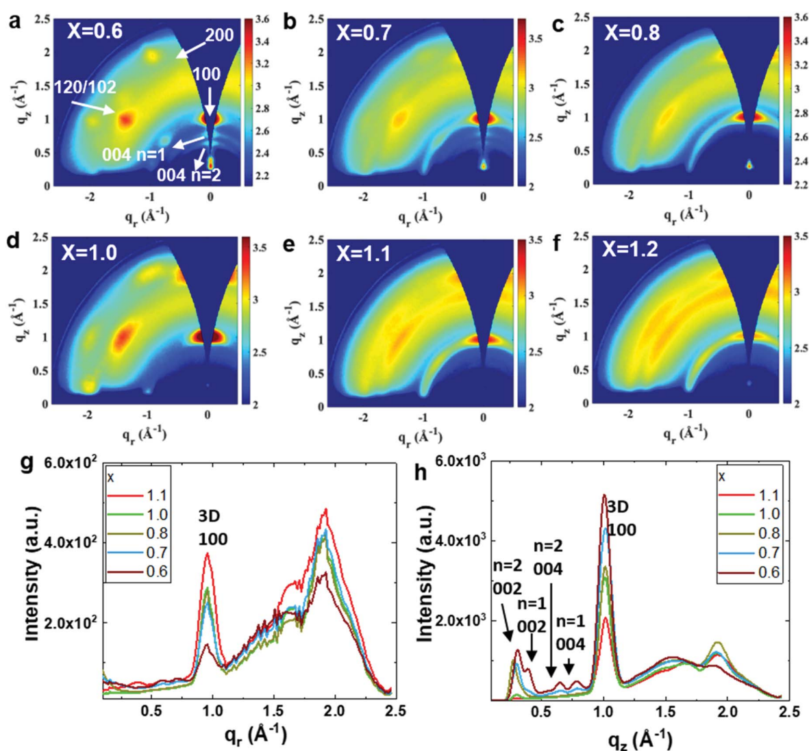
Fig. 2 GIWAXS patterns of (a) the PEA 0.08 FA 0.6 SnI 3 , (b) PEA 0.08 FA 0.7 SnI 3 , (c) PEA 0.08 FA 0.8 SnI 3 , (d) PEA 0.08 FA 1.0 SnI 3 , (e) PEA 0.08 FA 1.1 SnI 3 and (f) PEA 0.08 FA 1.2 SnI 3 films. The images were recorded using an incident angle of 2^\circ . Line-cut data of the PEA 0.08 FA x SnI 3 ( x = 0.6-1.1 ) films along (g) q_r and (h) q_z directions.
