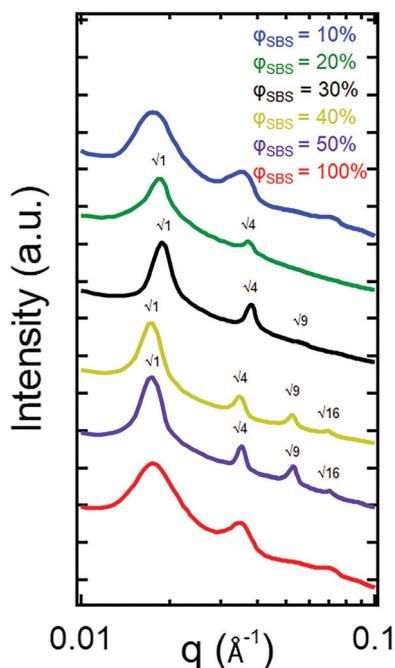
Fig. 4 1D SAXS patterns for the dog bone samples after polymerization and vacuum drying. A transition to LAM is seen with samples \phi_{\text{SBS}} = 50\% , 40%, 30%, and 20% from the higher-order reflections indexed to the primary scattering peak as indicated on the scattering curves. Scattering plots have been vertically shifted.
