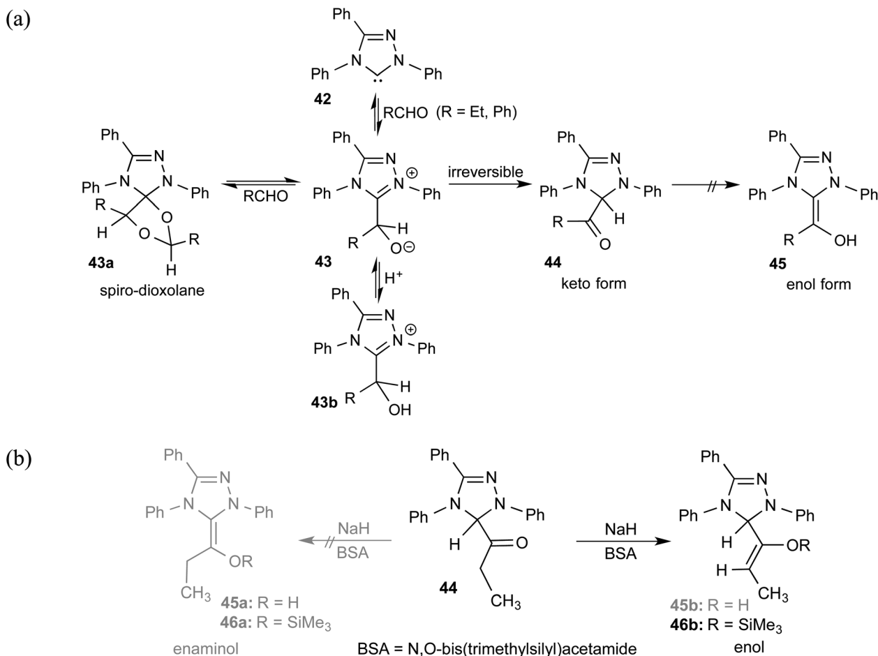
Scheme 10 (a) Generation of the keto- and enol-tautomers and spiro-dioxolane from a triazolyliene carbene and an aliphatic aldehyde. (b) The formation of the keto-tautomer of the Breslow intermediate.
