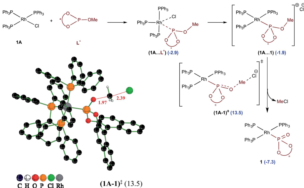
Scheme 2 (a) The relative Gibbs free energies of the formation (in \text{kcal mol}^{-1} ) of different likely active species computed with respect to the separated reactants. (b) Important steps in the conversion of Rh-bound BINOL-methyl phosphite to the corresponding phosphonate ligand through the Rh-Arbuzov rearrangement and a representative example of an optimized geometry for the expulsion of methyl chloride. Any of the active catalysts listed here is assigned a general notion 1 when it is considered in the catalytic cycle as shown in Scheme 3.
