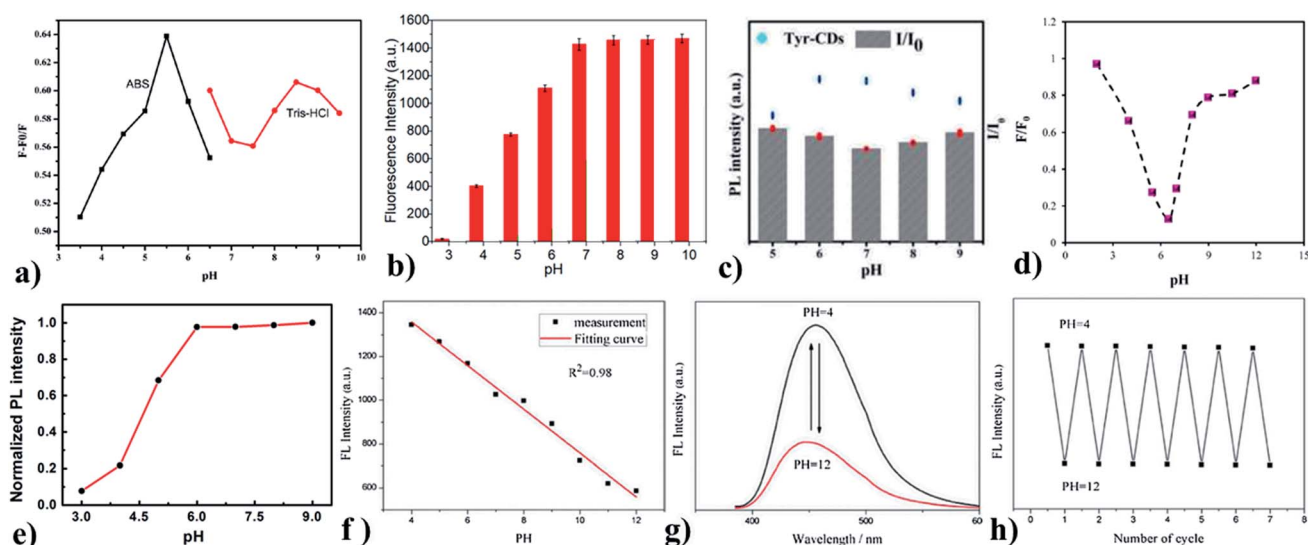
Fig. 4 (a) and (b) pH vs. change in fluorescence intensity of Gly-GQDs, (c) pH vs. change in the fluorescence intensity of Tyr-CDs, (d) pH vs. change in fluorescence intensity of Val-GQDs, (e) pH vs. change in the fluorescence intensity of L-CQDs, (f) pH vs. change in the fluorescence intensity for BR buffer, (g) pH vs. fluorescence spectra of Trp-GQDs, (h) Response of reversible fluorescence for varying pH cycles. In the figure, (a) has been reproduced from ref. 79 with permission from Elsevier, copyright 2017; (b) has been reproduced from ref. 33 with permission from Elsevier, copyright 2021; (c) has been reproduced from ref. 80 with permission from Elsevier, copyright 2015; (d) has been reproduced from ref. 34 with permission from Elsevier, copyright 2017; (e) has been reproduced from ref. 81 with permission from Springer, copyright 2016; (f)–(h) have been reproduced from ref. 84 with permission from Elsevier, copyright 2019.
