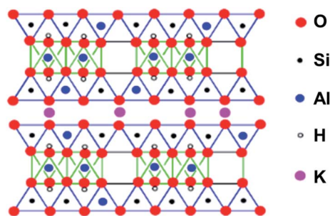
Fig. 7 The structure of a mica, muscovite, (\text{KF})_2(\text{Al}_2\text{O}_3)_3(\text{SiO}_2)_6(\text{H}_2\text{O}) . The space between the layers is occupied only by \text{K}^+ ions. The layer structure facilitates cleavage to produce flat surfaces. Adapted from https://employees.csbsju.edu/cschaller/PrinciplesChem/network/NWalumina.htm (accessed 17 th November 2020), courtesy of Chris Schaller.
