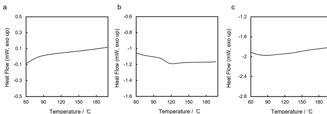
Fig. 4 DSC curves of (a) lin -poly( 1,4Si 6 ), (b) cyc -poly( 1,3Si 6 ), and (c) lin -poly( 1,3Si 6 ). The second cycle is shown. Heating rate: 3 °C min -1 for lin -poly( 1,4Si 6 ), 20 °C min -1 for cyc -poly( 1,3Si 6 ) and lin -poly( 1,3Si 6 ).
