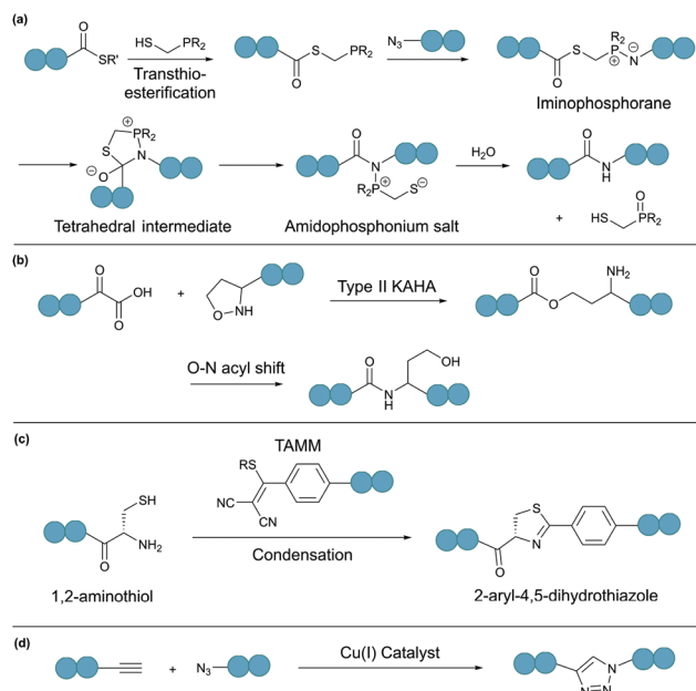
Fig. 4 Selected bioorthogonal reactions for peptide/protein cyclization: (a) traceless Staudinger ligation, (b) type II KAHA ligation, (c) TAMM condensation, and (d) CuAAC.
