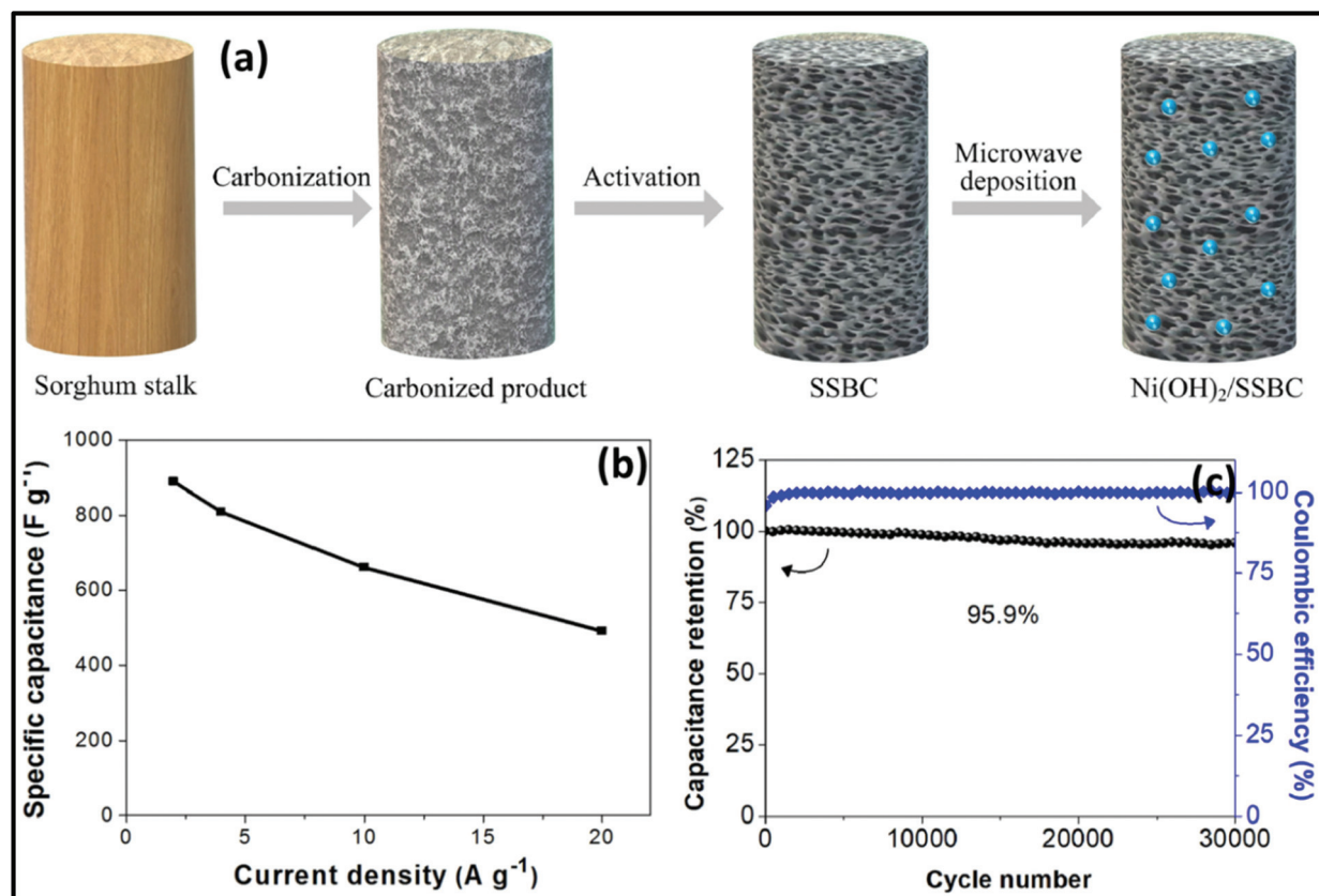
Fig. 18 (a) Synthesis of Ni(OH) 2 /sorghum stalk biomass carbon, (b) specific capacitance of Ni(OH) 2 /sorghum stalk biomass carbon composite and (c) cyclic property and coulombic efficiency of Ni(OH) 2 /sorghum stalk biomass carbon composite. Reprinted (adapted) with permission from ref. 267, copyright (2020), Elsevier B.V. All rights reserved.
