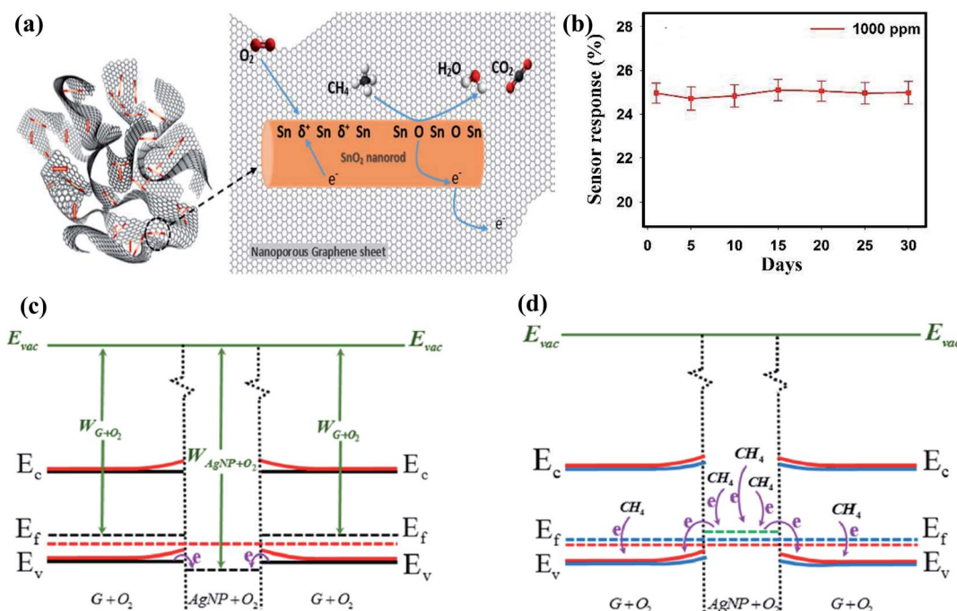
Fig. 9 (a) Schematic representation of sensing mechanism for CH 4 detection on SnO 2 -graphene-based sensor. (b) Stability graph of sensor (response calculated using \Delta R/R_a ) 45 (reprinted with permission from ref. 45, Copyright (2017), with permission from Elsevier). (c) Schematic illustration of the energy band diagrams for preadsorbed graphene and Ag NPs under ambient conditions. (d) Electron transfer upon exposure to CH 4 (ref. 87) (reprinted with permission from ref. 87, Copyright (2019) American Chemical Society).
