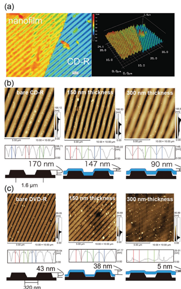
Fig. 7 (a) Laser microscope images of the edge of the [(Ala) 10 -PPG] m nanofilm (300 nm thick) on a CD-R surface. (b) and (c) AFM images of bare and [(Ala) 10 -PPG] m nanofilms (150 nm and 300 nm thick)-coated CD-R (b) and DVD-R (c) surfaces and their corresponding height profiles.
