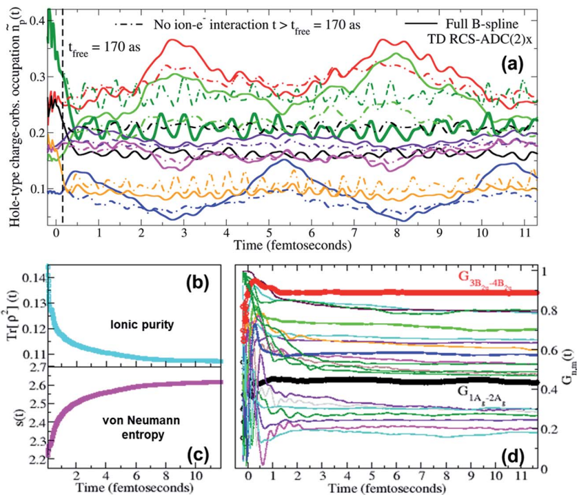
Fig. 5 (a) Time-dependent hole-occupation numbers \bar{n}_p(t) (eqn (11)) of the “occupied” natural charge orbitals triggered by attosecond ionisation of the C 4 H 4 N 2 molecule in the pump step; full lines: full TD RCS-ADC(2)x results; dashed lines: results obtained by switching off the residual interaction between the parent-ion and the photoelectron at t_{\text{free}} = 170 as after ionisation. Time evolution of (b) the purity \text{Tr}[\rho^2](t) and (c) the von Neumann entropy of entanglement s(t) of the bipartite ion–photoelectron system after pump ionisation of the C 4 H 4 N 2 molecule. (d) Time evolution, upon ionisation by the pump laser pulse, of the degrees of coherence G_{m,n}(t) of the pairs of ionic states mostly contributing to the density-matrix purification (see Fig. 6); the time evolution of the G_{1A_g, 2A_g}(t) (black curve) and G_{3B_{2u}, 4B_{2u}}(t) (red curve) coherences, mostly contributing to the pump-triggered charge dynamics, are highlighted.
