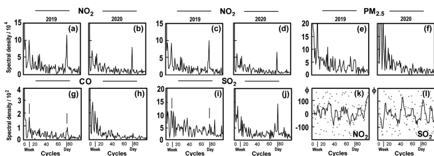
Fig. 3 Fourier transforms of hourly concentration data across Beijing for 75 days starting on 24th January: (a) \text{NO}_2 2019 within 5th Ring Road 2019, (b) \text{NO}_2 2020 within 5th Ring Road and across all the sites 2019, (c) \text{NO}_2 , (d) \text{NO}_2 , (e) \text{PM}_{2.5} 2019, (f) \text{PM}_{2.5} 2020, (g) CO 2019, (h) CO 2020, (i) \text{SO}_2 2019 and (j) \text{SO}_2 2020, and the phase angle, in degrees for (k) \text{NO}_2 within 5th Ring Road 2020 and (l) \text{SO}_2 2020, where the smoothed trend line added is a 5-point running mean. Note: the x-axis shows the number of cycles in the 75 day record, so 75 marks the daily cycle, and the weekly cycle is expected at 10–11 as marked. The y-axis in figures (a)–(j) denotes spectral power which takes the units of concentration squared. The y-axis in figures (k) and (l) is the phase angle in degrees.
