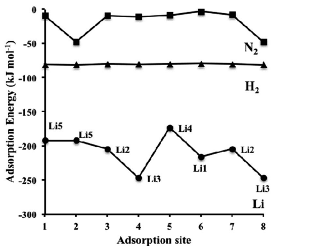
Fig. 8 Dispersion-corrected (revPBE-D3) adsorption energies of Li (circles), H_2 (triangles) and N_2 (squares) over the symmetry unique adsorption sites on \eta\text{-Mn}_3N_2 depicted in Scheme 1 (for H_2 and N_2 ). The data for Li corresponds to the adsorption site configuration depicted in Scheme 2. Lines connecting the data points have been drawn to guide the eye.
