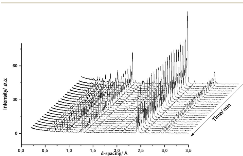
Fig. 3 Diffraction patterns of \theta\text{-Mn}_6\text{N}_{5+x} during the discharge reaction at 400 °C. In situ measurements were conducted under 60 \text{ mL min}^{-1} 75 vol% \text{H}_2 in Ar (BOC, 99.98%). Patterns were collected for 10 min.
