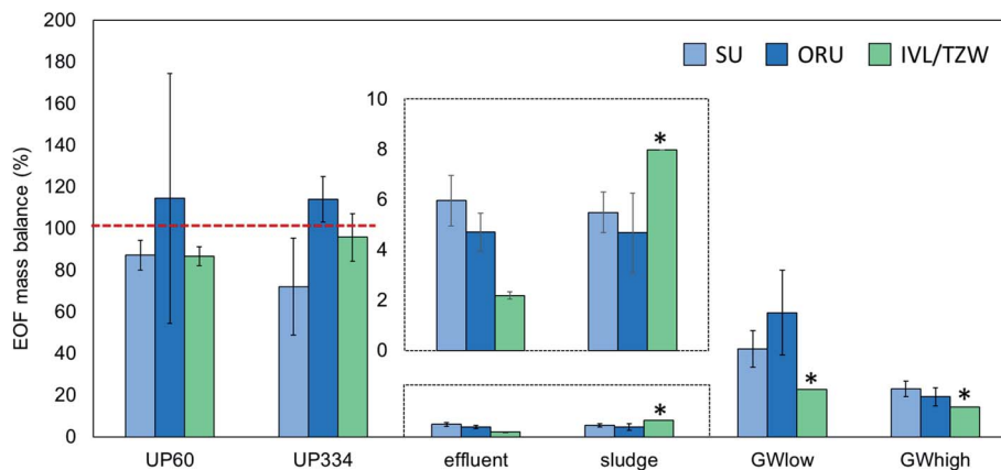
Fig. 2 EOF mass balance (%) in interlaboratory comparison samples. Error bars represent pooled standard deviation ( n = 3 for EOF and \Sigma PFAS-16). The dashed red lines indicate the expected EOF mass balance. * indicates that only a single measurement was performed.
