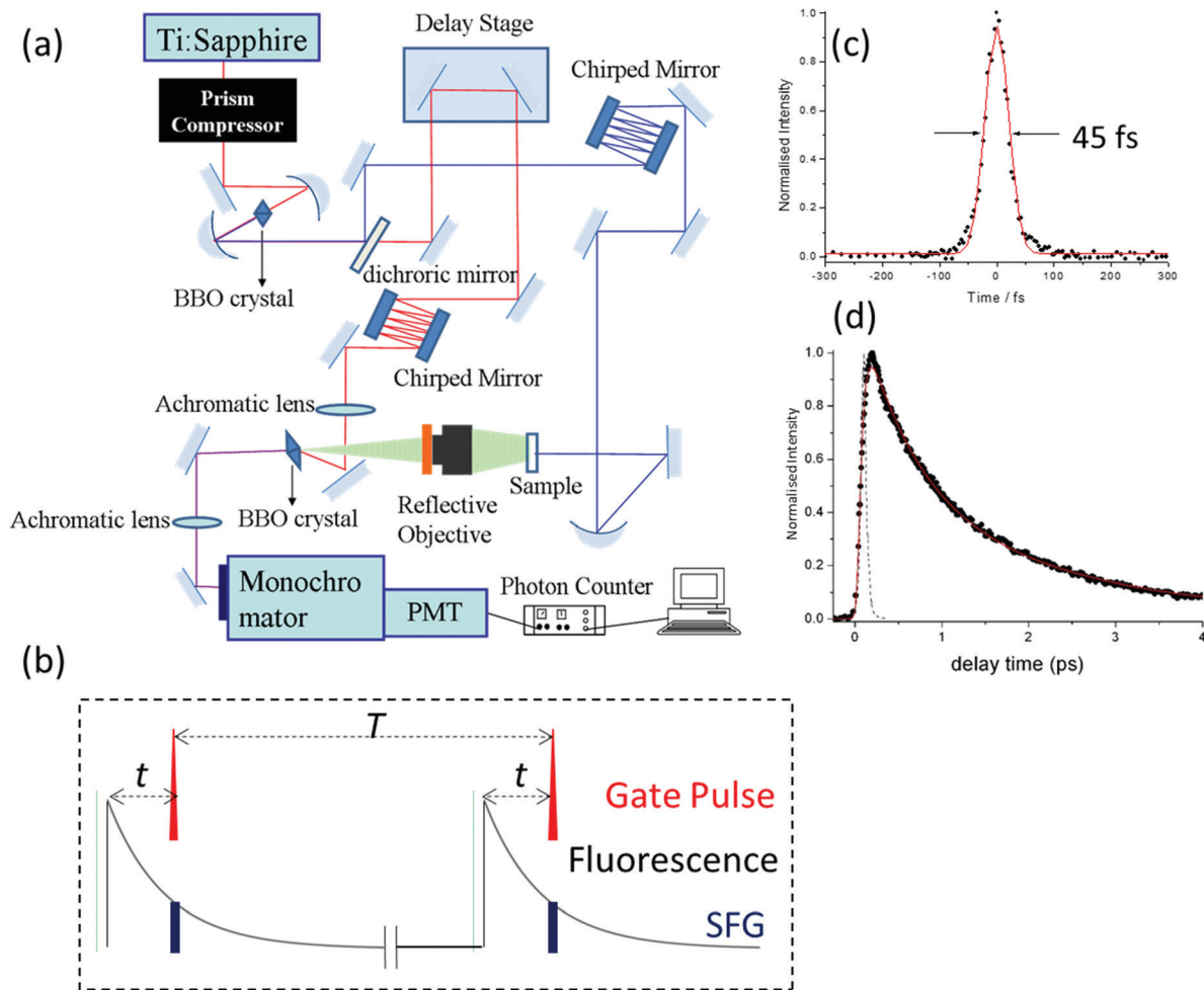
Fig. 1 Fluorescence up-conversion. (a) Experimental layout, BBO = beta-barium borate nonlinear crystals, PMT = low noise photon counting photomultiplier. (b) Cartoon of the basic measurement. The fluorescence is mixed with the gate pulse in the BBO crystal. The up-conversion intensity is proportional to the instantaneous intensity of the fluorescence, which is measured as a function of gate delay, t . (c) Cross correlation of pump and gate pulses from up converted pump Raman scatter from heptane, fit to a 45 fs width Gaussian function. (d) Example of a measured decay with subpicosecond lifetime.
