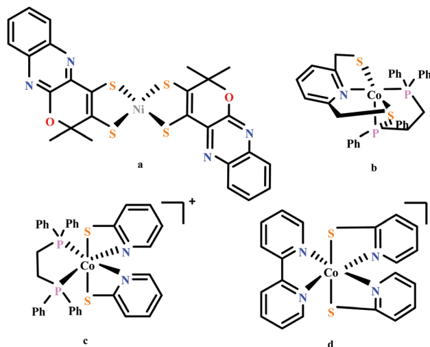
Fig. 9 Representative metal-thiolate based electrocatalysts for \text{CO}_2 reduction.
