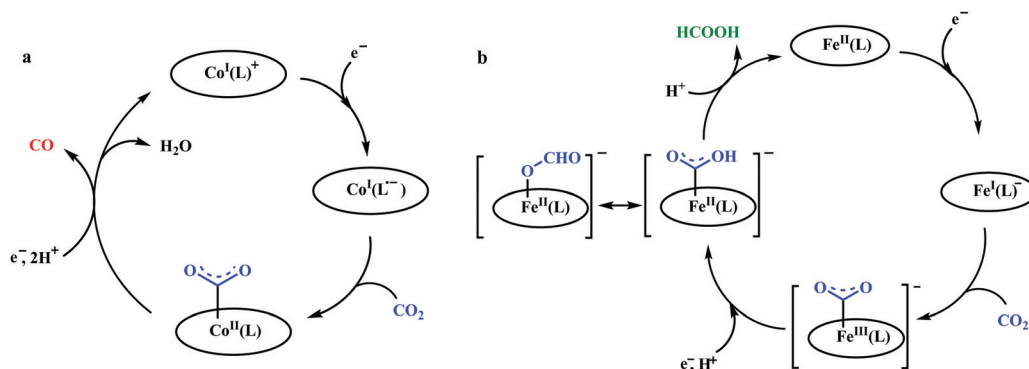
Scheme 14 Proposed mechanistic pathway for electrocatalytic \text{CO}_2 reduction to CO vs. formic acid; catalyzed by same ligand framework but with different metals: (a) cobalt and (b) iron.
