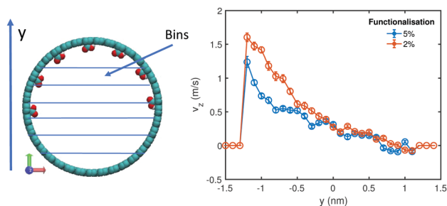
Fig. 6 Velocity profiles for the systems shown in Fig. 5.
