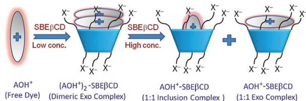
Scheme 8 Schematic representation of the multistep binding interactions of acridine orange dye (AOH + ) with changing SBEβCD host concentration. The scheme has been reproduced from ref. 37 with permission from the Royal Society of Chemistry.
