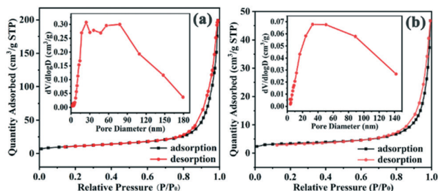
Fig. 9 \text{N}_2 adsorption-desorption isotherms and corresponding pore size distributions (inset) of (a) the \text{Cu}_2\text{O} hollow spheres and (b) \text{Cu}_2\text{O} nanocages.
