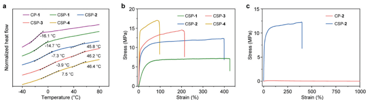
Fig. 4 (a) DSC curves of CP-1 and CSPs-1–4 recorded by heating scan from -40 to 80 °C with a heating rate of 20 °C \text{min}^{-1} . (b) Tensile stress–strain curves of CSPs-1–4 in the bulk. Deformation rate: 20 mm \text{min}^{-1} . (c) Tensile stress–strain curves of CP-2 and CSP-2 samples in the bulk. Deformation rate: 20 mm \text{min}^{-1} .
