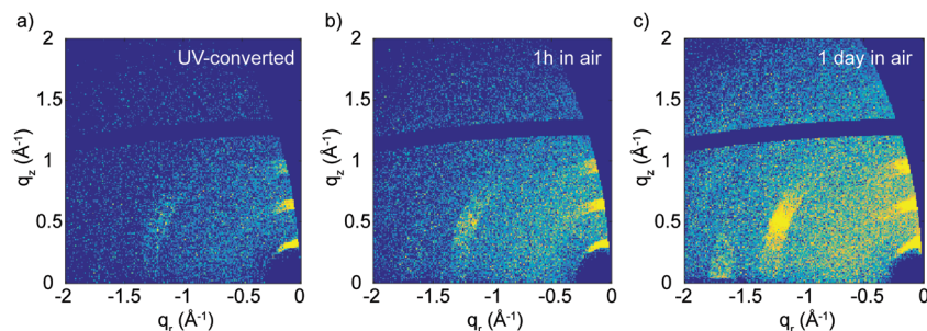
Fig. 4 Evolution of the GIWAXS patterns for the (\text{PEA})_2\text{CuCl}_4 film in air (a) just after irradiation with UV light, (b) 1 hour after irradiation and (c) 1 day after irradiation. The incident angle was 0.2°. Note that the sample was kept in the same place during this measurement, to ensure that a quantitative comparison between the different images can be made.
