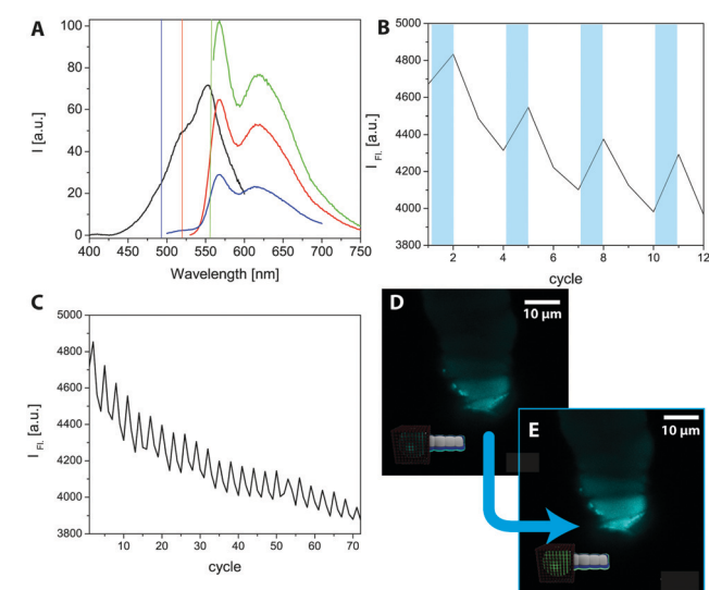
Fig. 4 (A) Excitation (black) and emission spectra of the synthesized compound 7 in ethanol. The vertical coloured lines correspond to the excitation wavelength (blue: 490 nm; red: 520 nm; green: 555 nm). (B) ROI (region of interest) intensity measurement over twelve scanning cycles on the LSM. Bleaching of the region (405 nm; 20% laser power; 4 scans; after the 1st and every third following cycle) is indicated as bluish areas. (C) Long-term cycling at the ROI over 72 cycles with the same settings chosen for B. (D) LSM image (excitation wavelength: 488 nm, 1% laser power) in false colours of a SP functionalized structure in the OFF (SP) state. (E) LSM image of a SP functionalized structure in the ON (MC) state.
