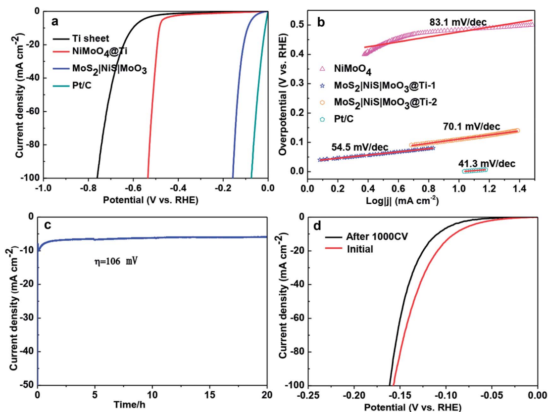
Fig. 4 (a) HER LSVs of MoS 2 |NiS|MoO 3 /Ti foil in comparison with other studied electrodes in 1 M KOH. (b) Corresponding Tafel plots. (c) CA response of MoS 2 |NiS|MoO 3 /Ti foil for more than 20 h. (d) HER LSVs of MoS 2 |NiS|MoO 3 /Ti foil before and after 1000 CV cycles. Reproduced with permission from ref. 60 (Copyright 2017 American Chemical Society).
