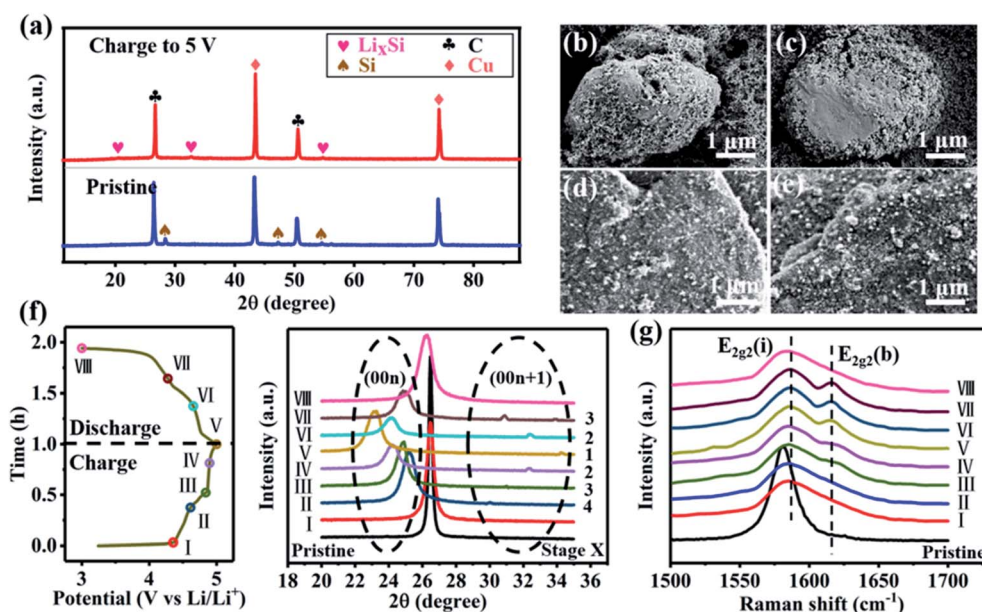
Fig. 5 (a) XRD patterns of the Si/C anode: pristine and charged to 5.0\text{ V} . (b and c) SEM images of the Si/C anode and (d and e) SEM images of the EG cathode before and after cycling. (f) The charging and discharging curves of the EG cathode at 100\text{ mA g}^{-1} and ex situ XRD patterns of EG, taken at various states of charging, as pointed out by the equivalent electrochemical curves. (g) Ex situ Raman patterns of EG, taken at various states of charging, as pointed out by the equivalent electrochemical curves.
