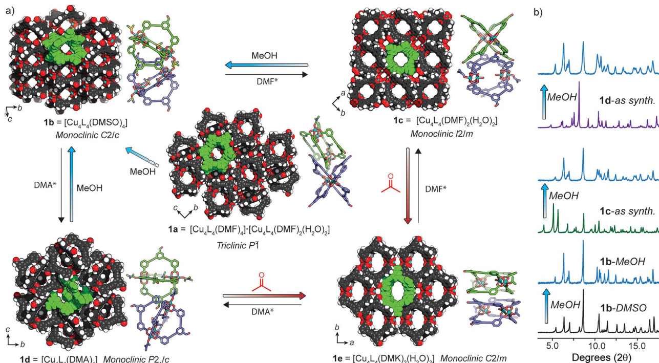
Fig. 3 (a) Single crystal X-ray structures of solvatomorphs 1a–e in a scheme portraying their structural transformations. The crystal packing of 1a–e is represented as space-filling (coordinating solvents removed for clarity) and alongside are depictions of the orientations of cage molecules within each phase. Each phase can be regenerated through recrystallisation (*co-solvent = \text{H}_2\text{O} ); (b) PXRD patterns highlighting the solid-state transformations of 1c and 1d \rightarrow 1b upon exposure to MeOH. Full details of the transformations shown in (a) can be found in the ESI (Fig. S11–S16†).
